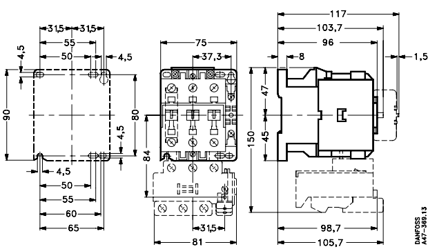
Contactors and motor starters CI 32, 37, 45, 50 Drilling dimensions
