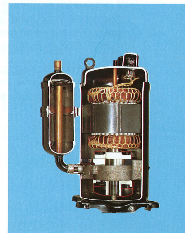
Cut-away view of RM5515GNVH
