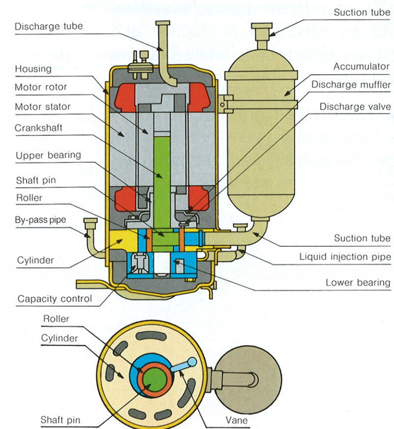
Interior design of rotary compressor with capacity control
