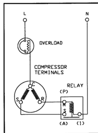
RSIR Motor Diagram with Current Relay
