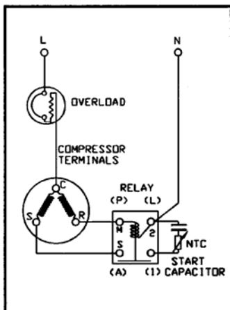
CSIR Motor Diagram with Current Relay
