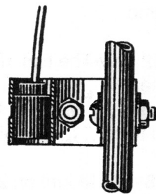
Section view of bulb mounted with the O18 strip clamp
