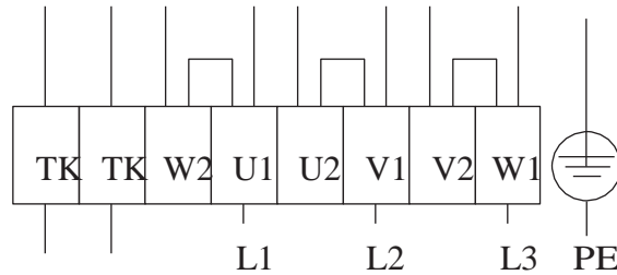
Δ: 连接 Δ: CONNECTION
