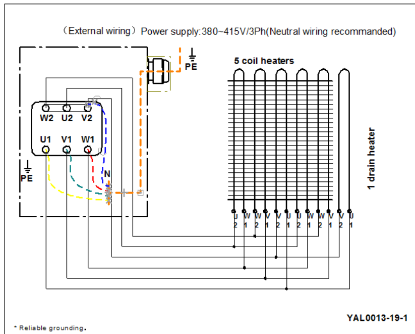
5 盘管加热器+1 排水盘加热器 5 Coil Heaters + 1 Drain Pan Heater
