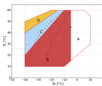
R448A/R449A- H33
