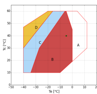
R407F- H33
