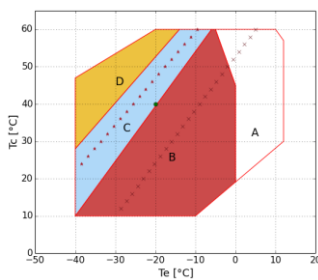
R407F- H33
