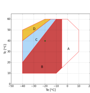
R448A/R449A- H33
