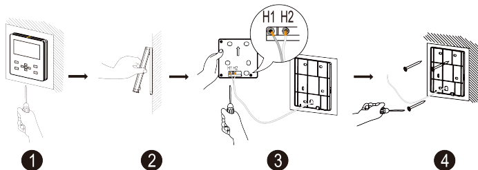
Figure 5-4 Disassembly Diagram for Wired Controller
