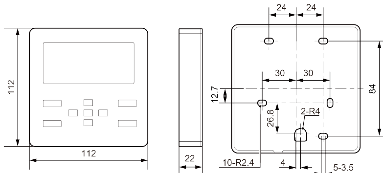
Figure 5-1 Dimension of Wired Controller
