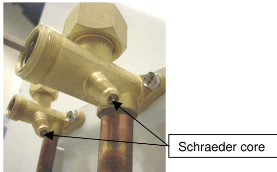
Typical service valves found on factory charged mini split A/C units. Note Schraeder cores are in place.
